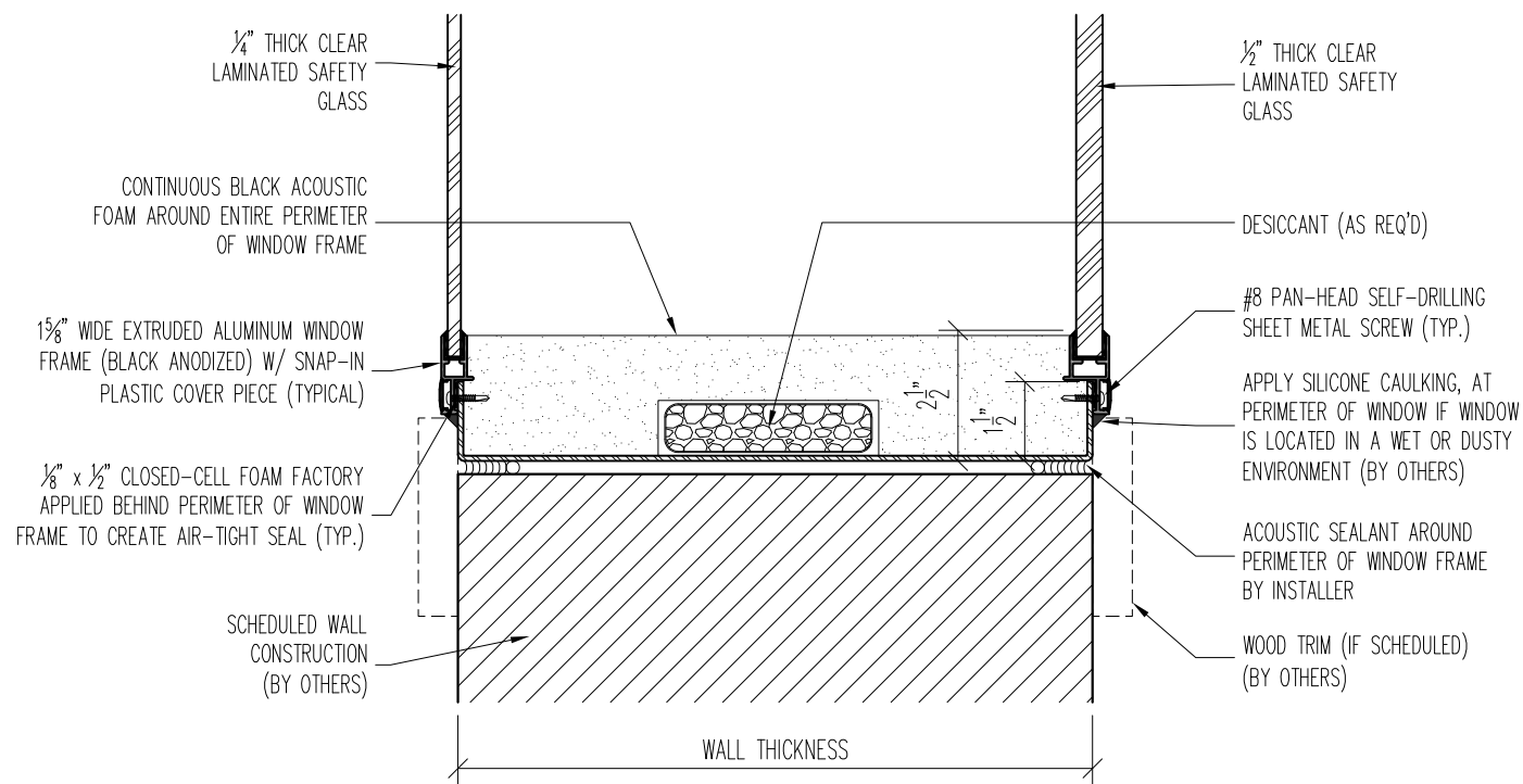
3 WS-2 ACOUSTIC WINDOW - SILL DETAIL
