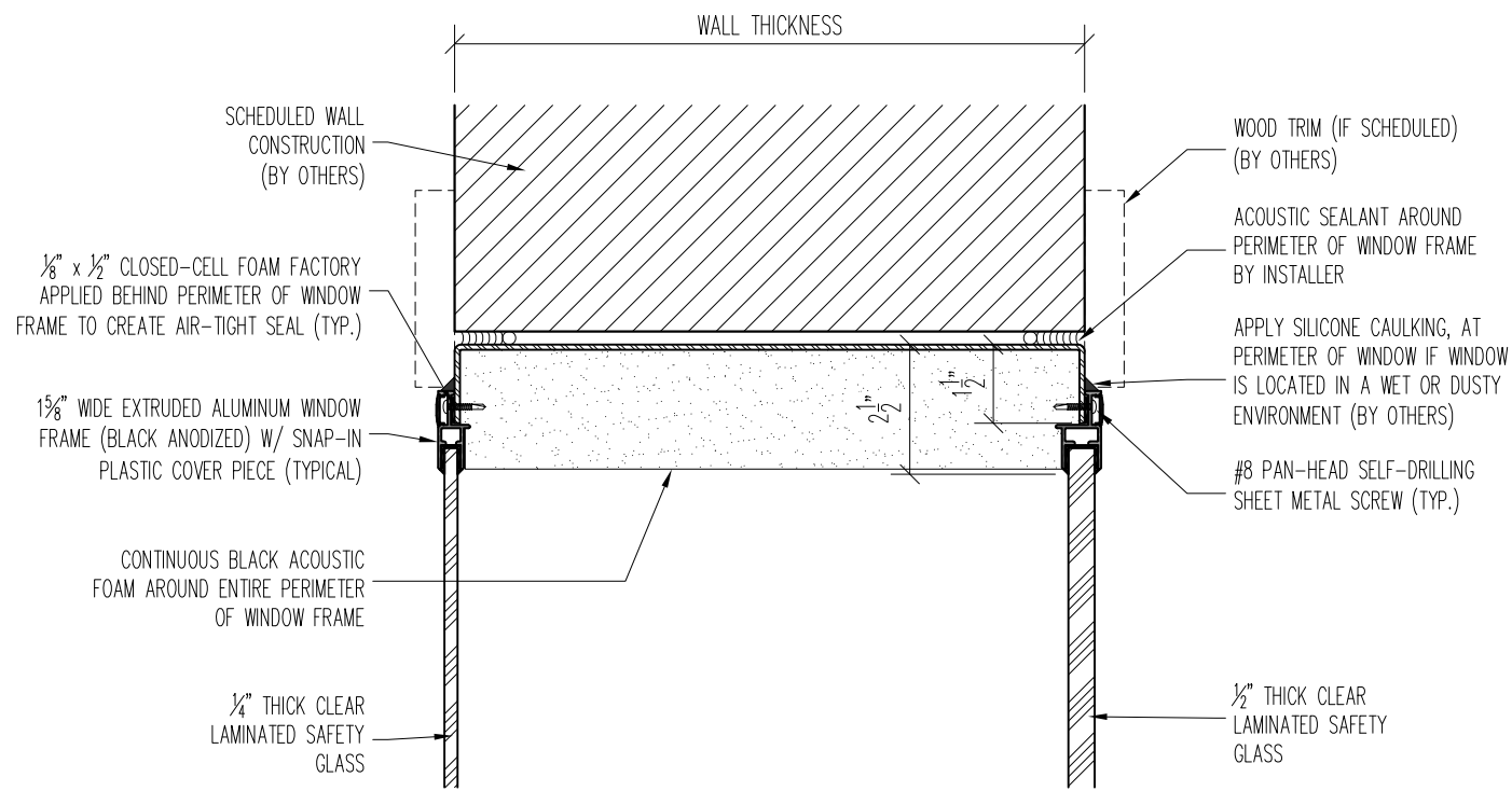
1 WS-2 ACOUSTIC WINDOW - HEAD DETAIL
