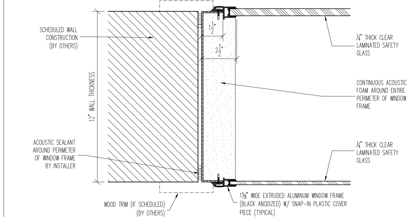
2 WS-2 ACOUSTIC WINDOW - JAMB DETAIL
