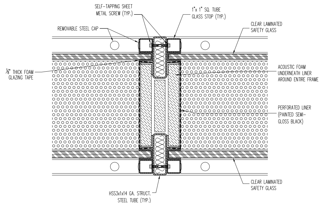
4 WS-2 ACOUSTIC WINDOW - MULLION DETAIL
