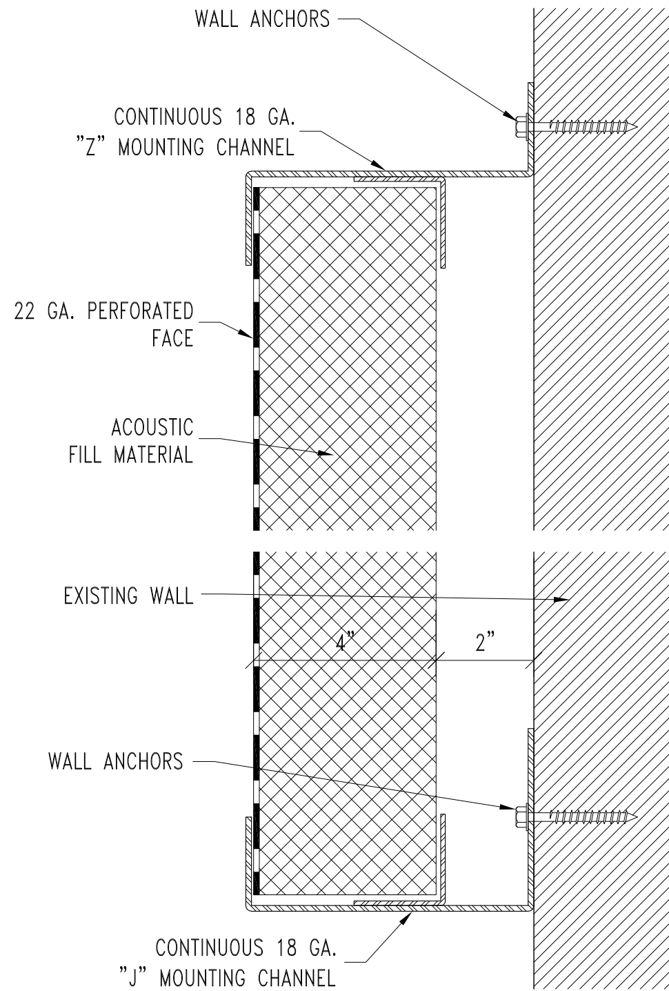
NB-IV PANEL W/ 2" OFFSET
