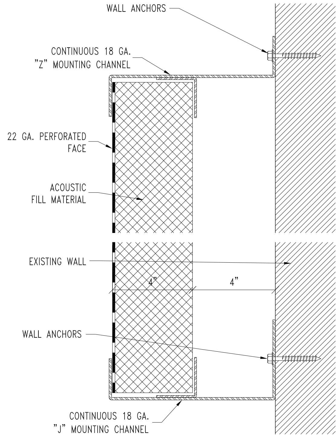
NB-IV PANEL W/ 4" OFFSET
