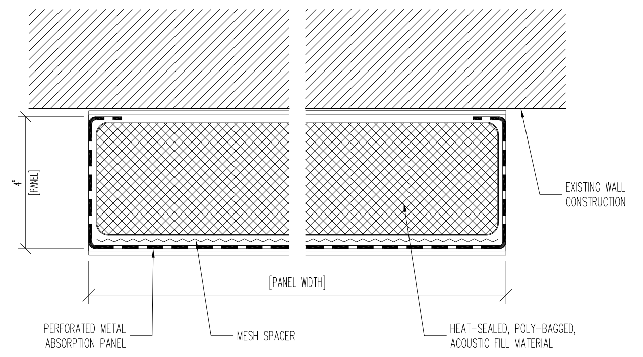
SECTION B-B
