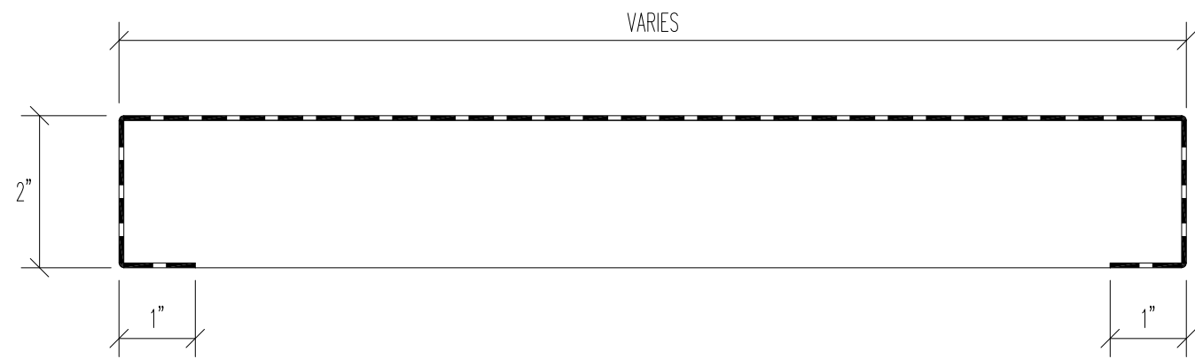
TYPICAL PANEL PROFILE
