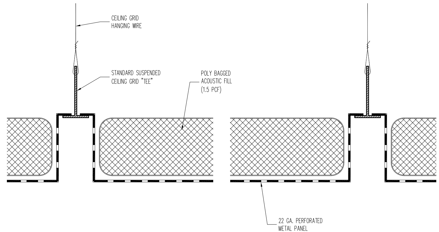
TYPICAL INSTALLATION SECTION DETAIL
