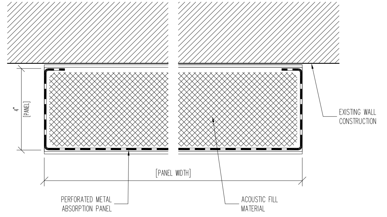
SECTION B-B
