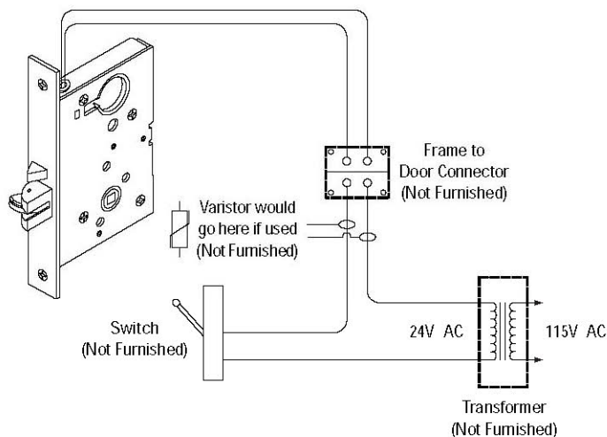
Typical Wiring Diagram for Electrified L-Series Locks
