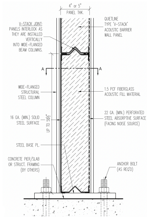
BARRIER WALLS SECTION DETAIL
