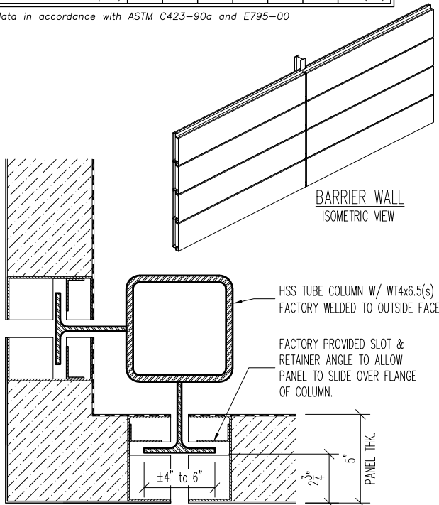
SECTION A-A - OPTION #1
