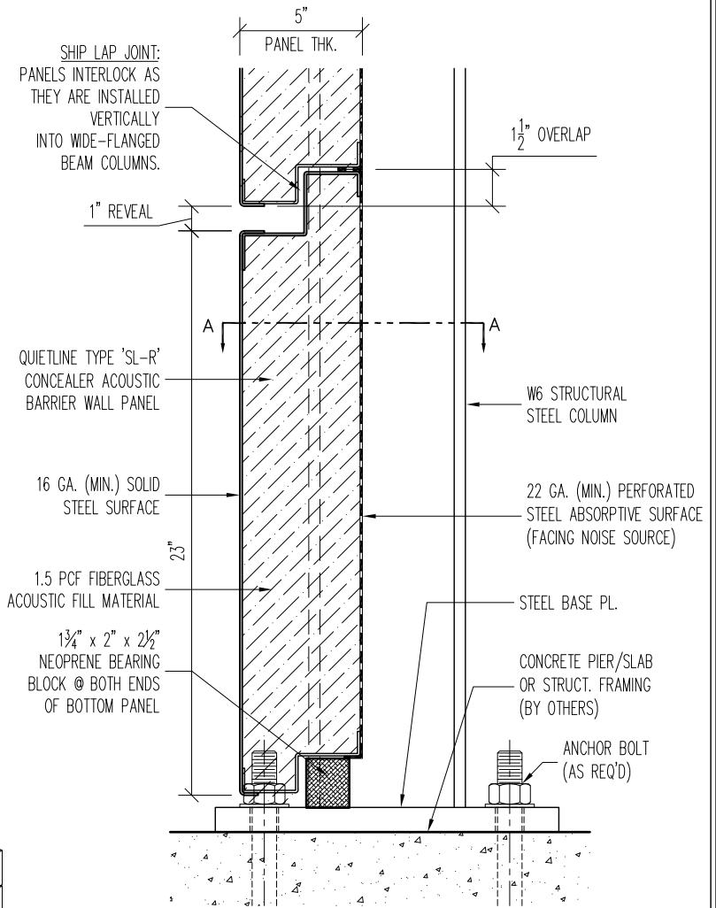
WALL SECTION DETAIL
