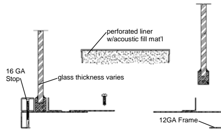
“Split-Frame” Design
