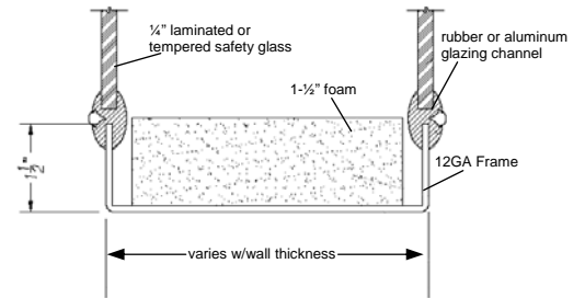
“U” Frame Design
