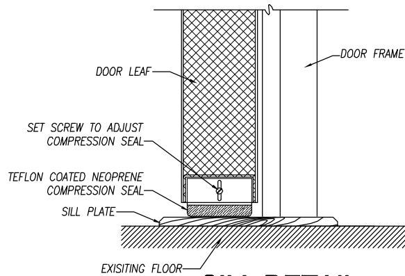
SILL DETAIL
