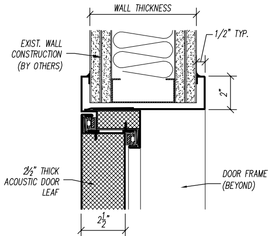
HEAD DETAIL
