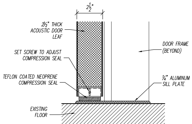
SILL DETAIL
